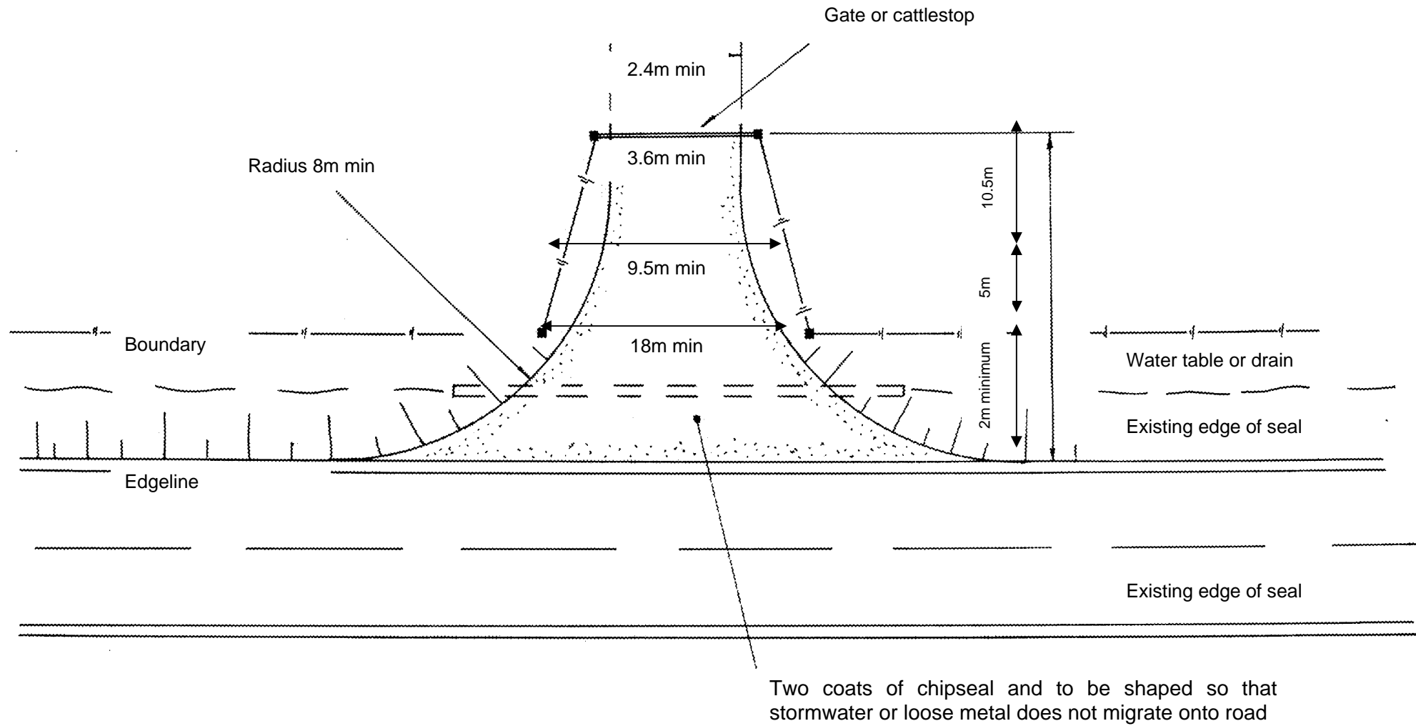
VEHICLE ENTRANCE FOR PROPERTIES NOT ON STATE HIGHWAYS (Diagram B)
