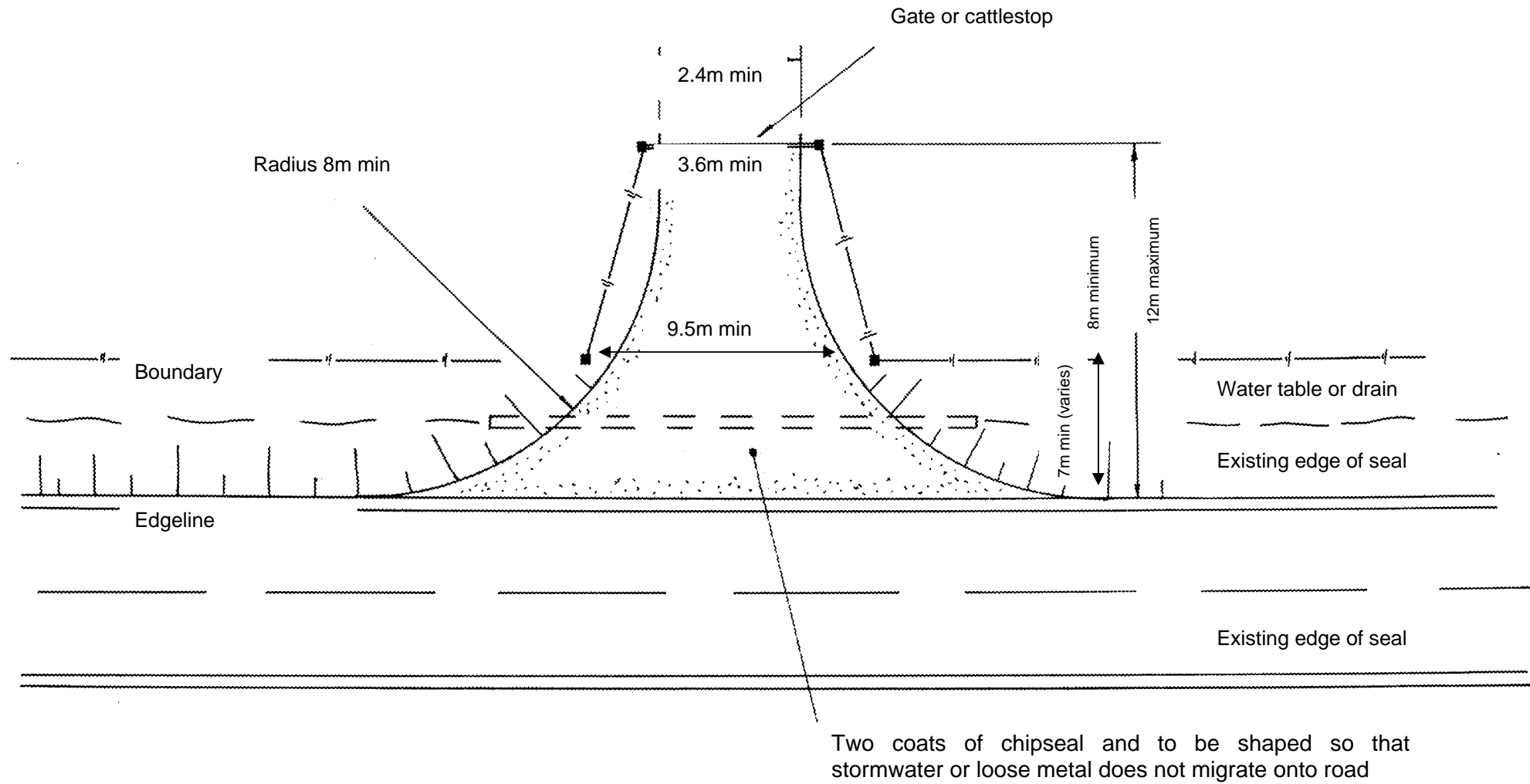
VEHICLE ENTRANCE TO PROPERTIES NOT ON STATE HIGHWAYS (Diagram A)
